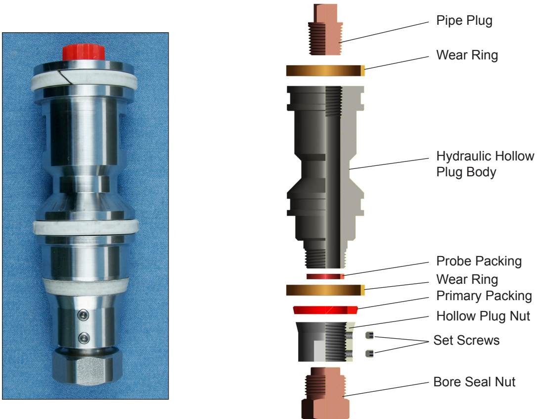
Hydraulic Hollow Plug Assembly HA700961158
